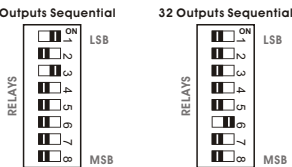
Fig. 4. How to program Outputs nº.
