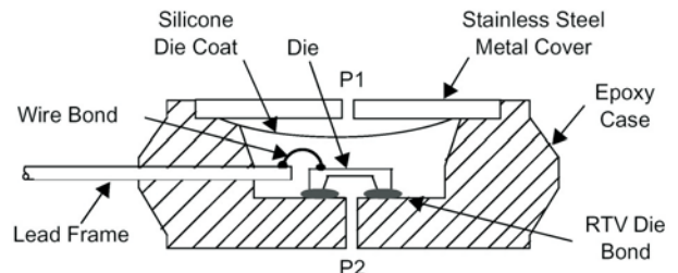
Figure 4. Cross-Sectional Diagram (not to scale)
