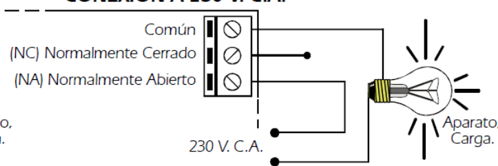
CONEXION A 230 V. C.A.
