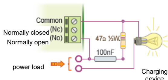
Fig 2 filter anti-relay fluctuations 230V AC load from 50W
