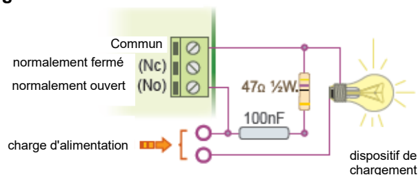
Fig 2 filtres anti-relais fluctuations 230V AC charges de 50W
