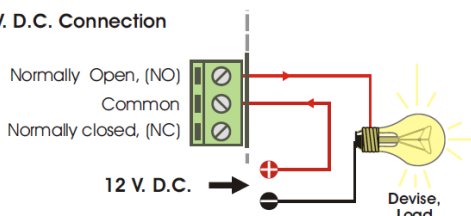
Fig. 1. Load Connection.
