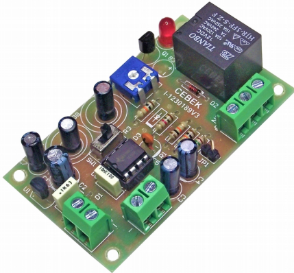
I-1 Universal timer to 12VDC - 50 mA. Time scale 0.1 second to 4 minutes.
