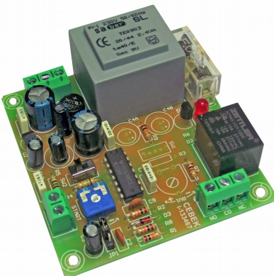
I-137 Delay timer start-up 230VAC. Time scale 8 seconds to 45 minutes.
