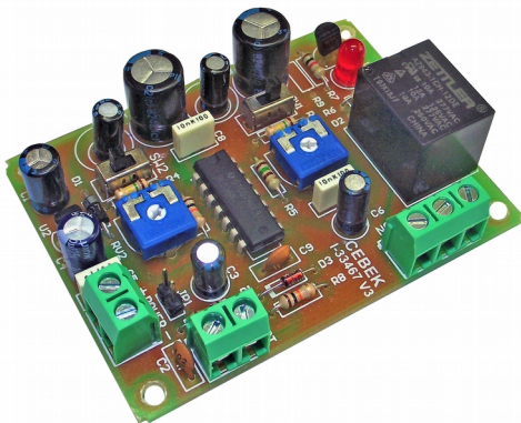
I-34 Delay Timer 12VDC - 60 mA. Time scale 8 seconds to 45 minutes.
