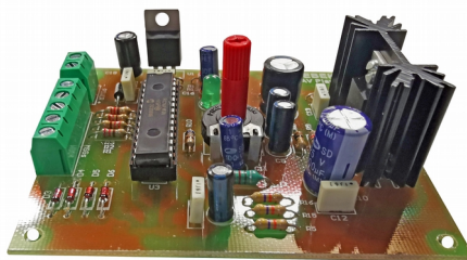
TR-30 WAV file player with 12VDC micro SD.
