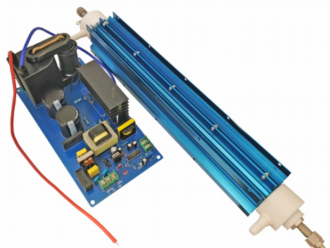
C-6891T Ozone generator with 20 gr / hour transformer.
