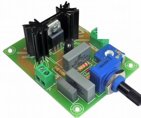
230VAC speed regulator
